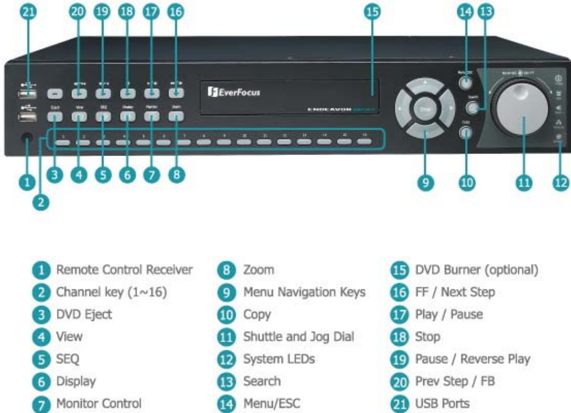
Figure 1-1 Front Panel
